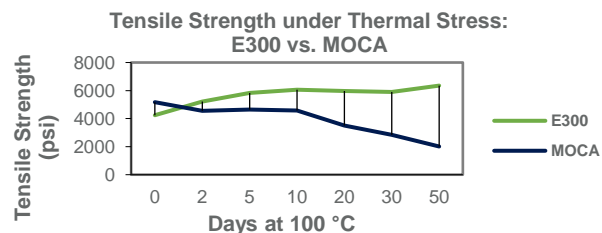
Figure 2: E300 vs. MOCA Thermal Aging
